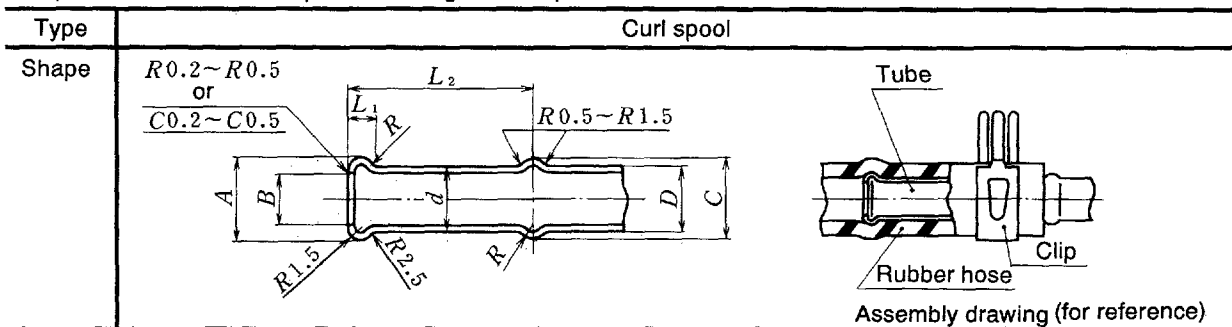
Attached table 7 Shape and dimensions of curl spool for tubing
