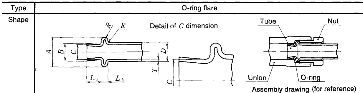
Assembly drawing (for reference)
