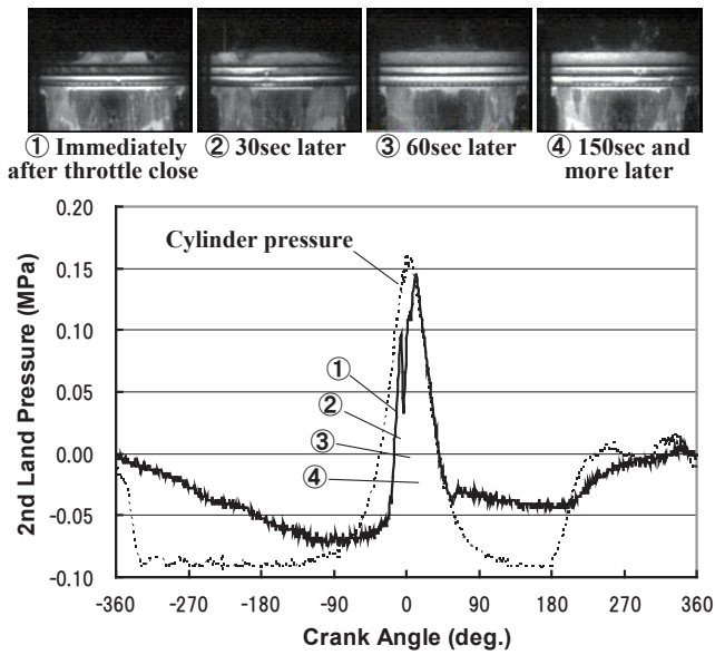
Fig. 13 2nd land pressure and oil behavior under transient state from the moment throttle closed (measured)
